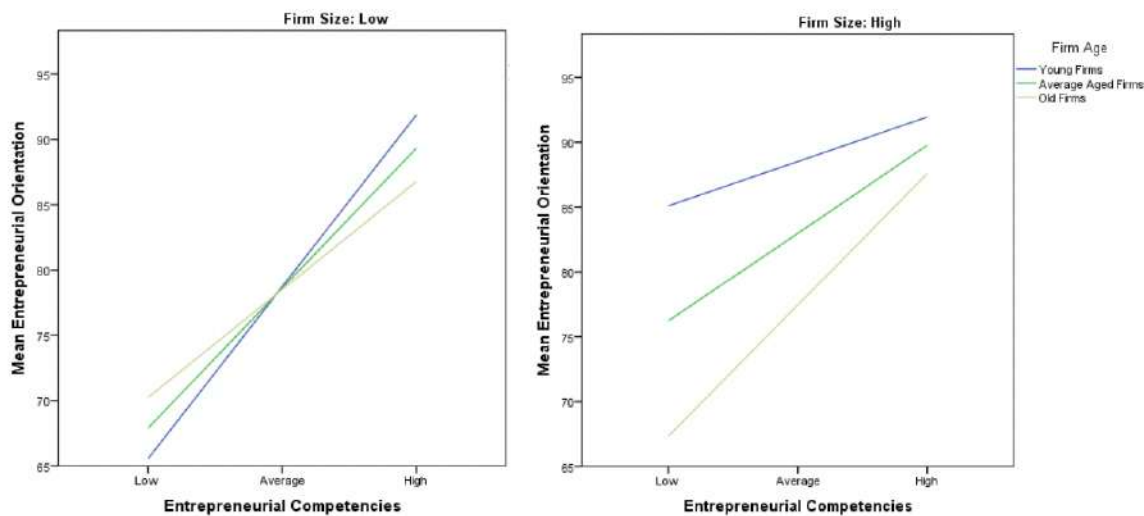
Figure 1 - Interaction Plots
